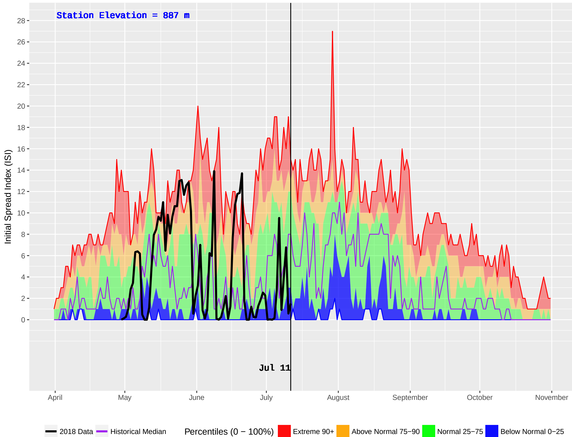
CRAWFORD (873) : Historical (2004–2016) and Current (2018) Noon Initial Spread Index (ISI)
