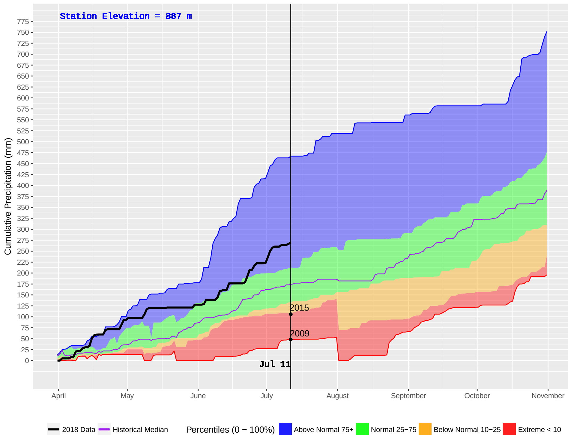
CRAWFORD (873) : Historical (2004–2016) and Current (2018) Noon Cumulative Precipitation
